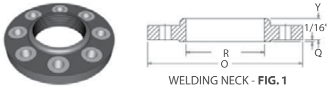
WELDING NECK - FIG. 1
