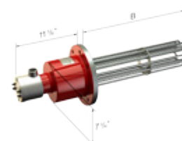
5 inch ANSI flanged NEMA 7
