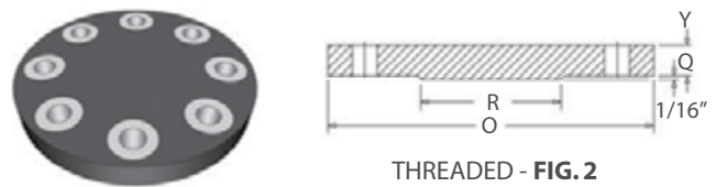
THREADED - FIG. 2
