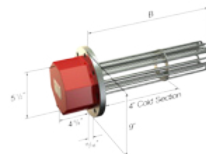
3 inch ANSI flanged heater NEMA 7
