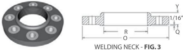
WELDING NECK - FIG. 3
